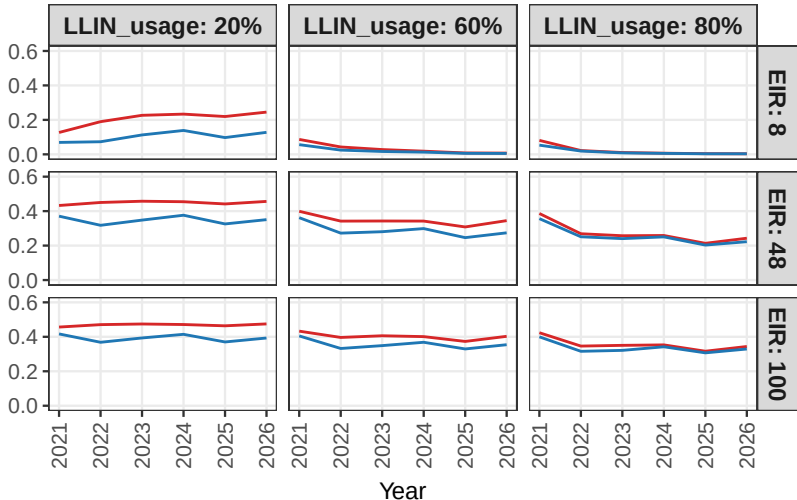
Malaria prevalence
